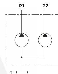
Hydraulic circuit
