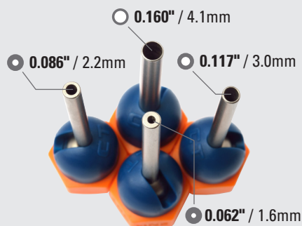
FOUR NOZZLE DIAMETERS Available on both CT and XR Nozzles
