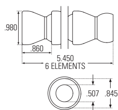
1/2" SYSTEM
