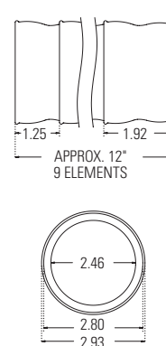
2-1/2" SYSTEM
