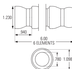
3/4" SYSTEM
