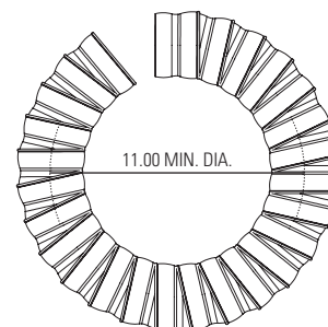
2-1/2" SYSTEM
