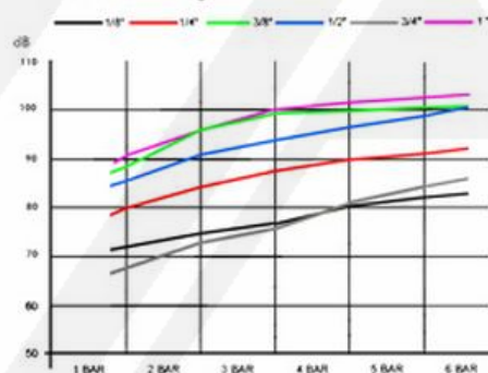
Acoustic fading
